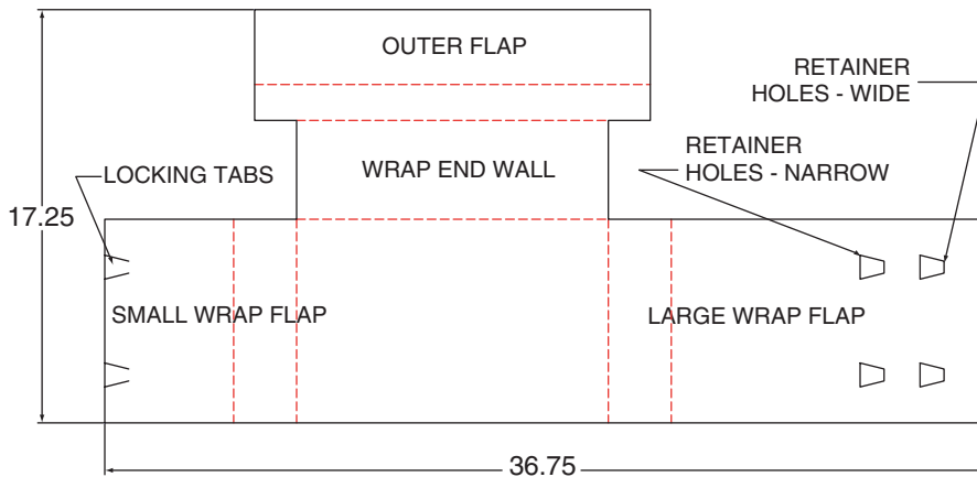
TOP VIEW OF RIGHT INNER PACK FOLDER FOR 4 LAMP PUFF
