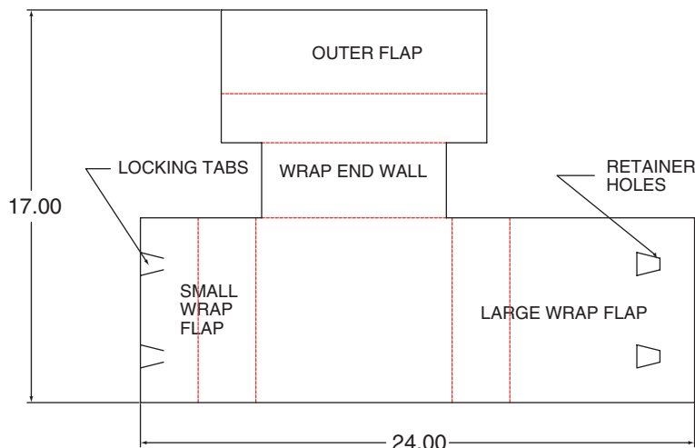
TOP VIEW OF RIGHT INNER PACK FOLDER FOR 2 LAMP PUFF
